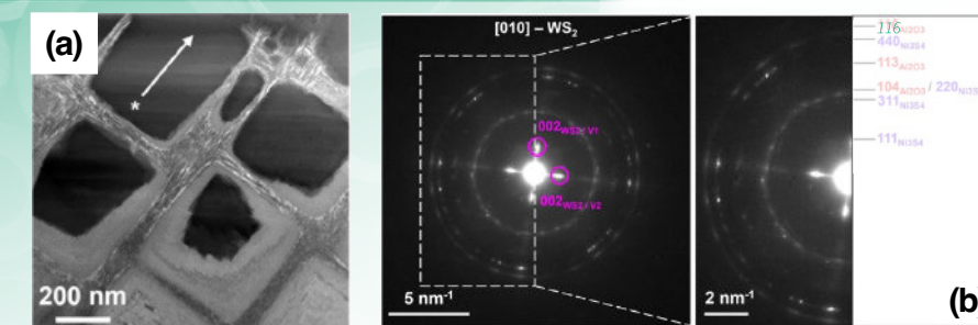
(a) Bright field STEM micrograph of the oxidation front of DS200+Hf after 100 h of exposure at 600°C in air + 400 ppm SO 2 , and (b) corroded \gamma/\gamma' microstructure: selected area electron diffraction (SAED) pattern and indexation of SAED.
